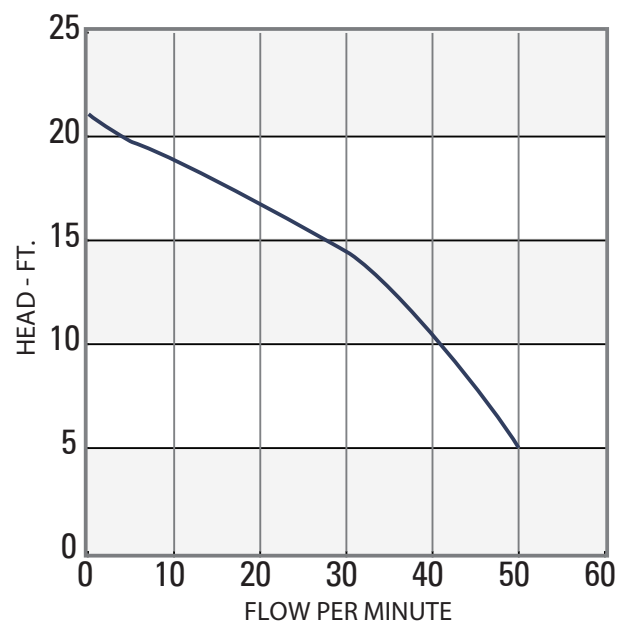
MODEL 3CD
