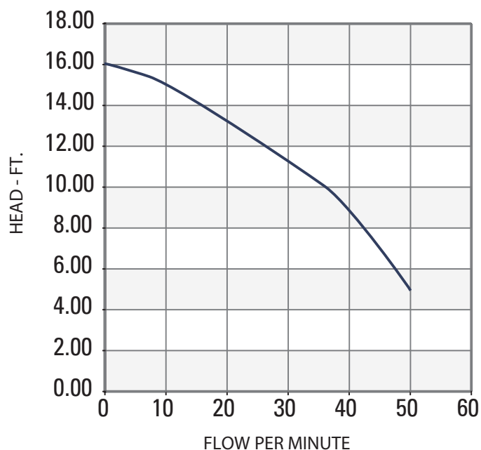
MODEL 3CE
